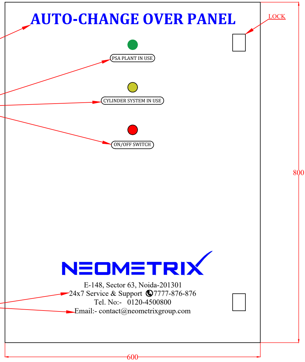
FRONT VIEW
