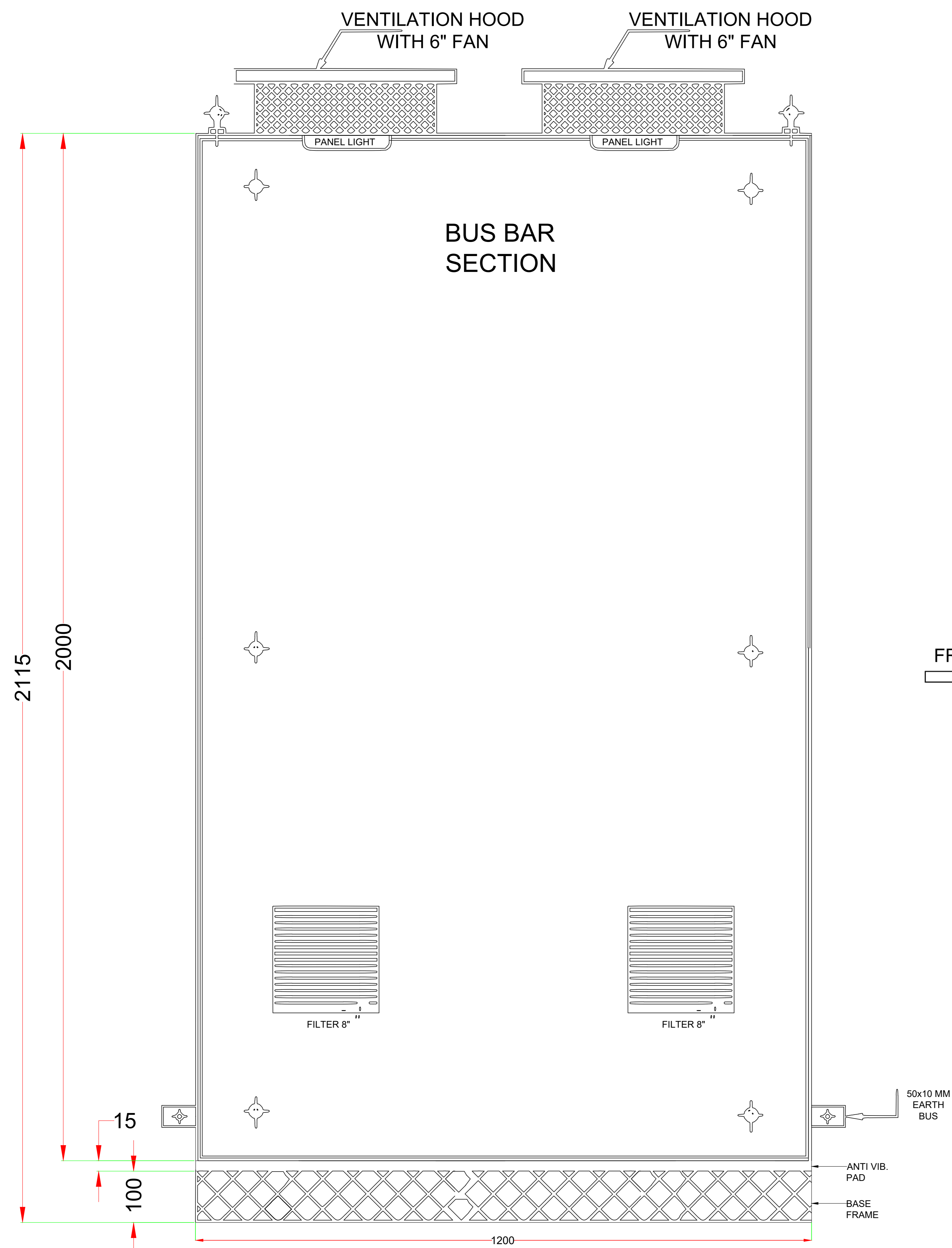
REAR VIEW EXTERNAL
