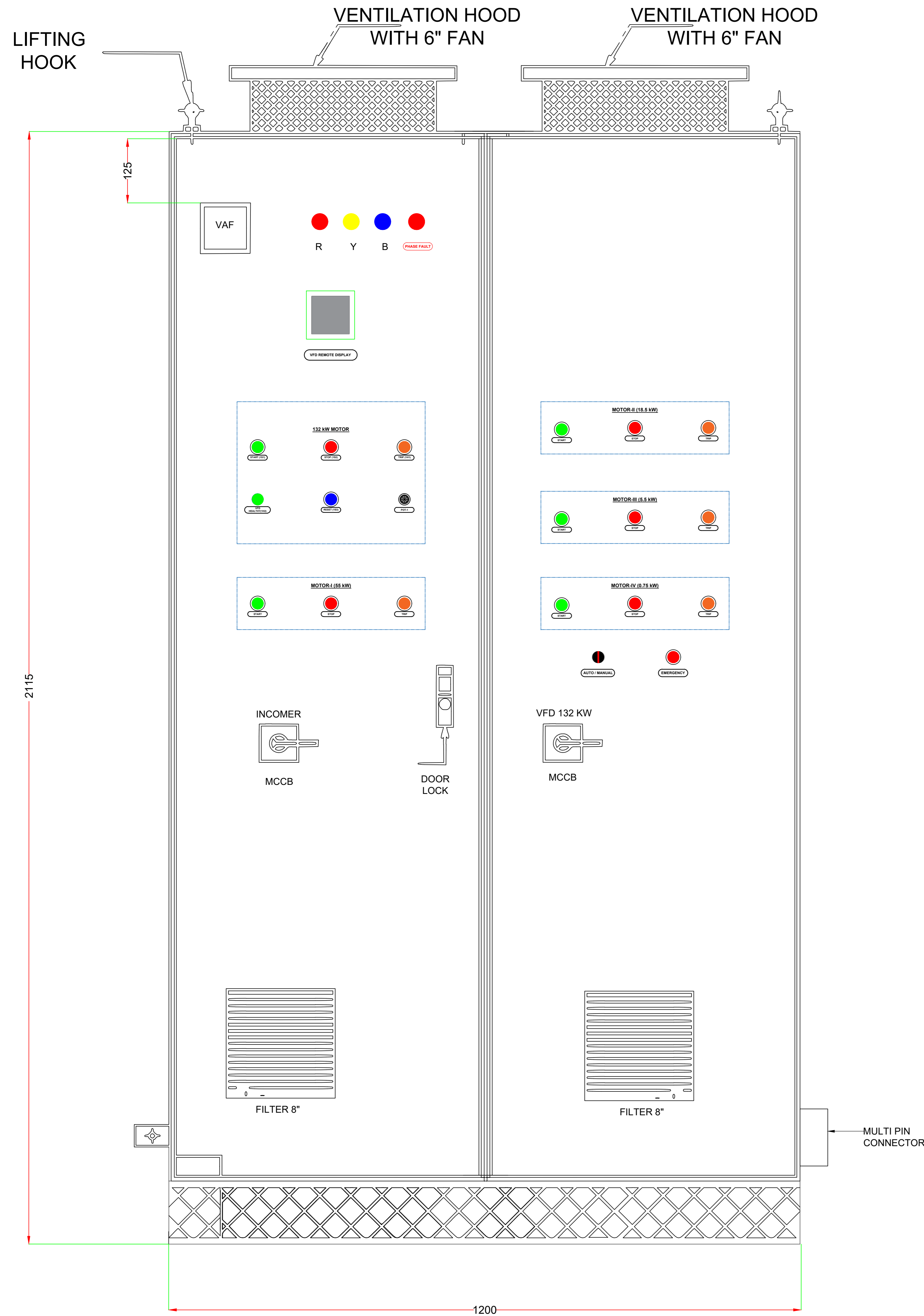
FRONT VIEW EXTERNAL
