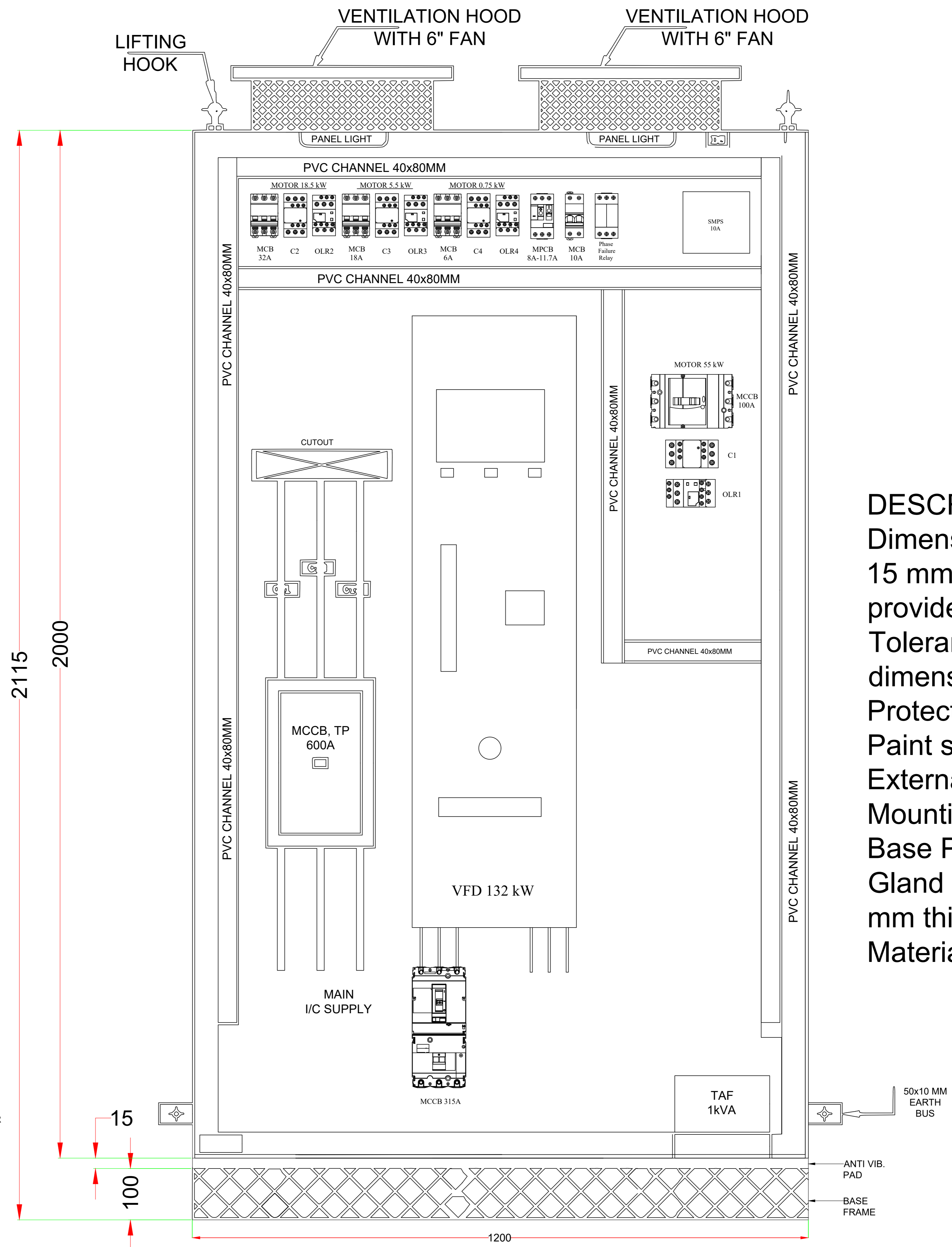
FRONT VIEW INTERNAL
