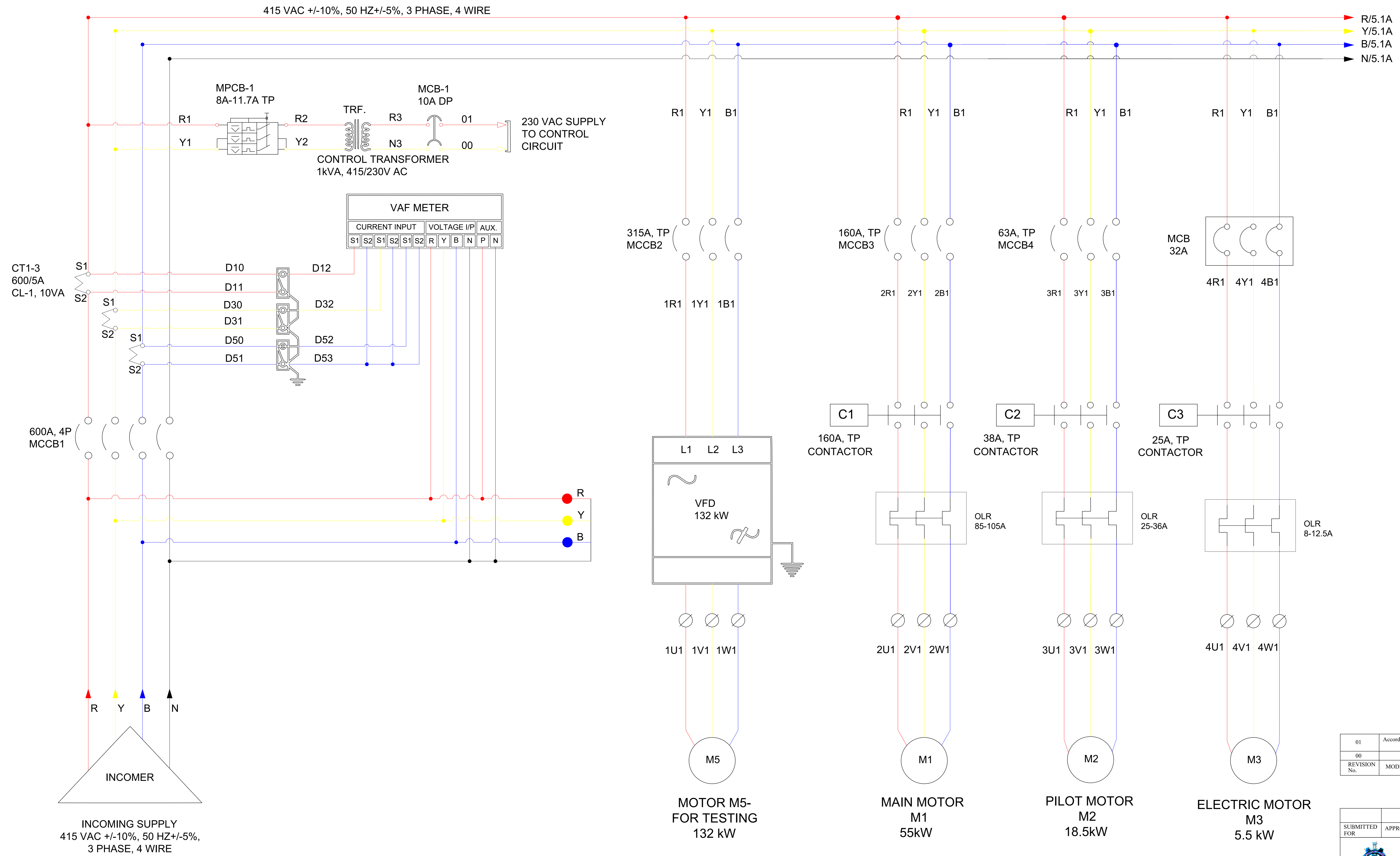
POWER WIRING DIAGRAM-I
