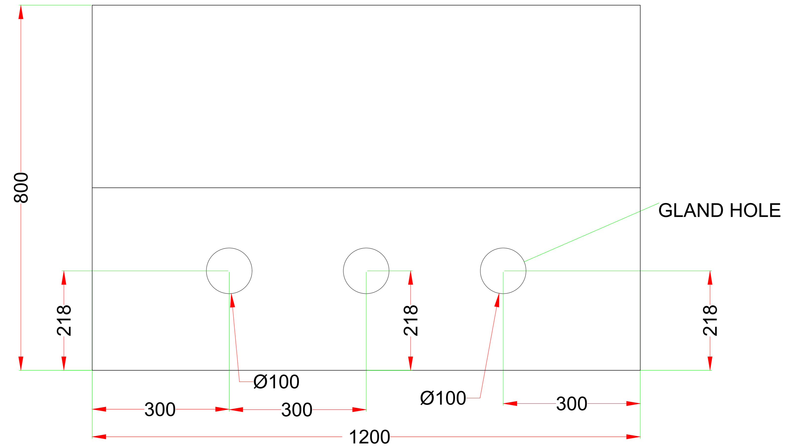
BOTTOM VIEW
