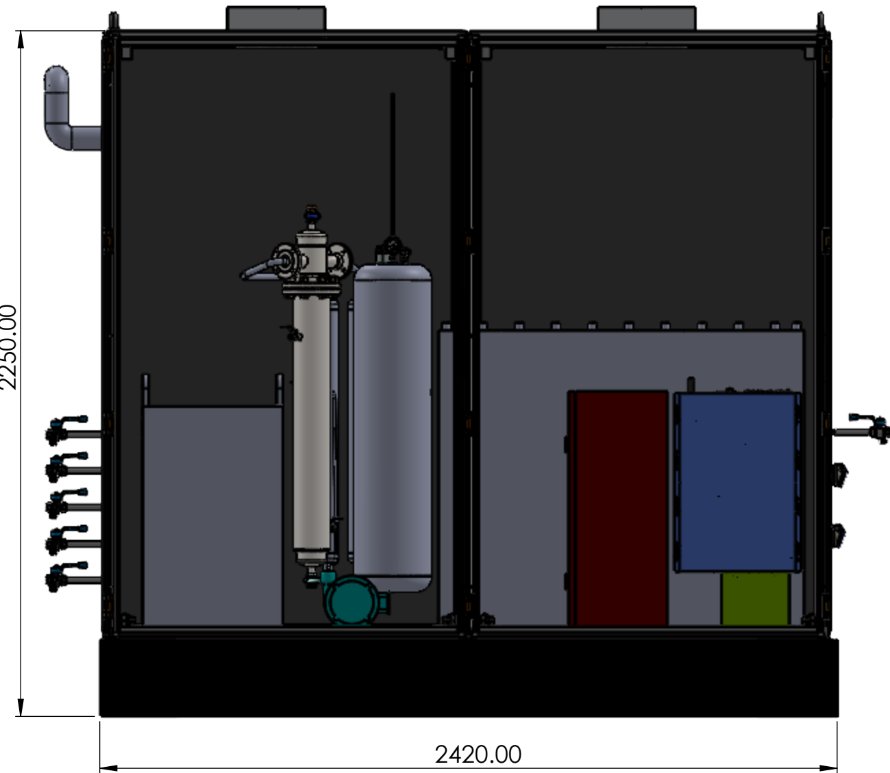
SIDE VIEW
