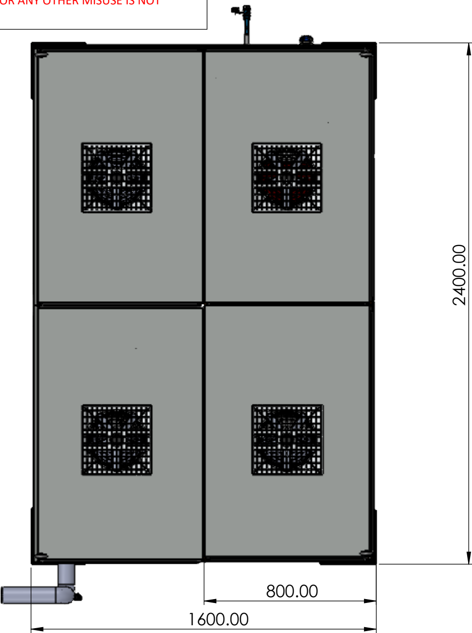
TOP VIEW
