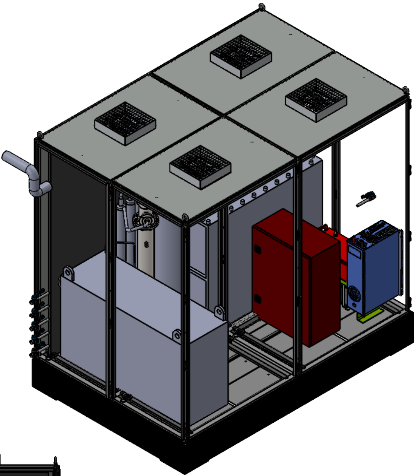
ISOMETRIC VIEW
