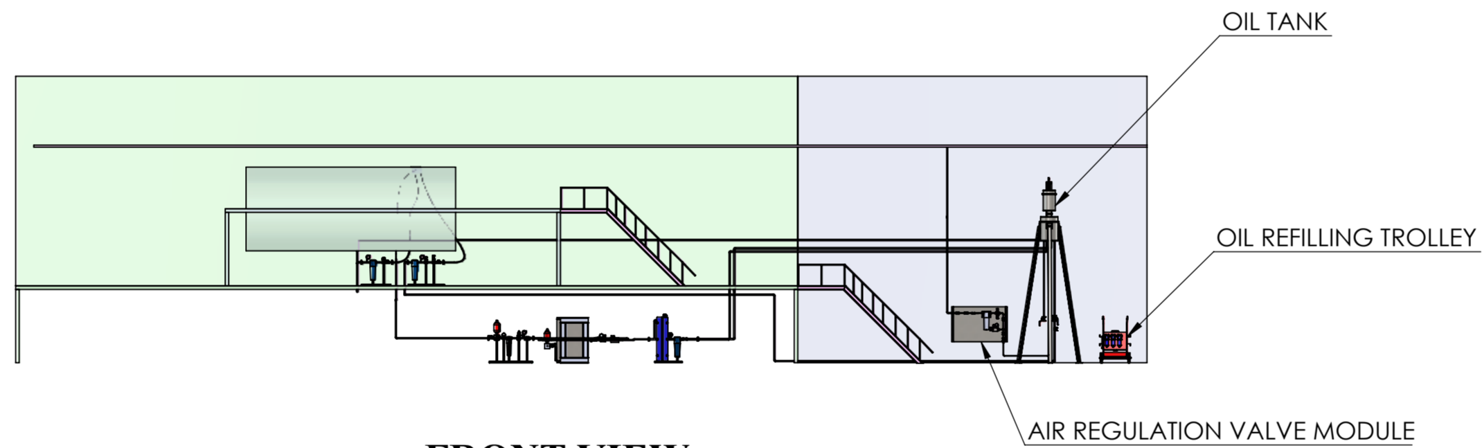
FRONT VIEW
