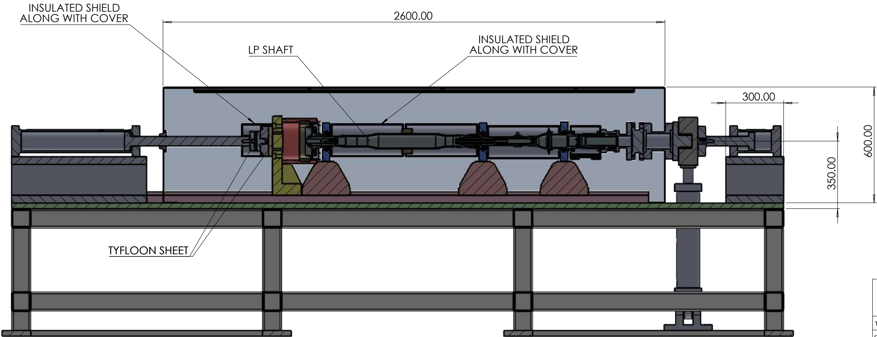
SECTION C-C SCALE 1 : 12
