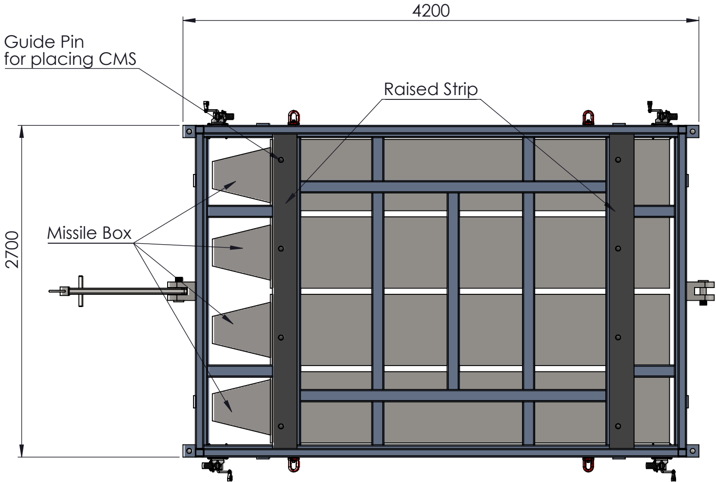
TOP VIEW
