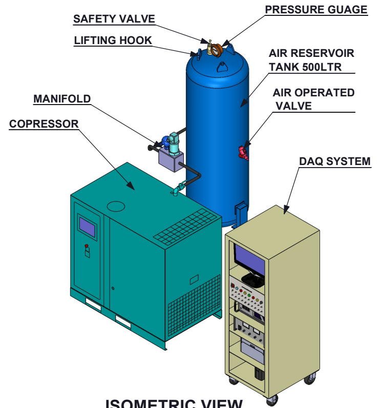
ISOMETRIC VIEW
