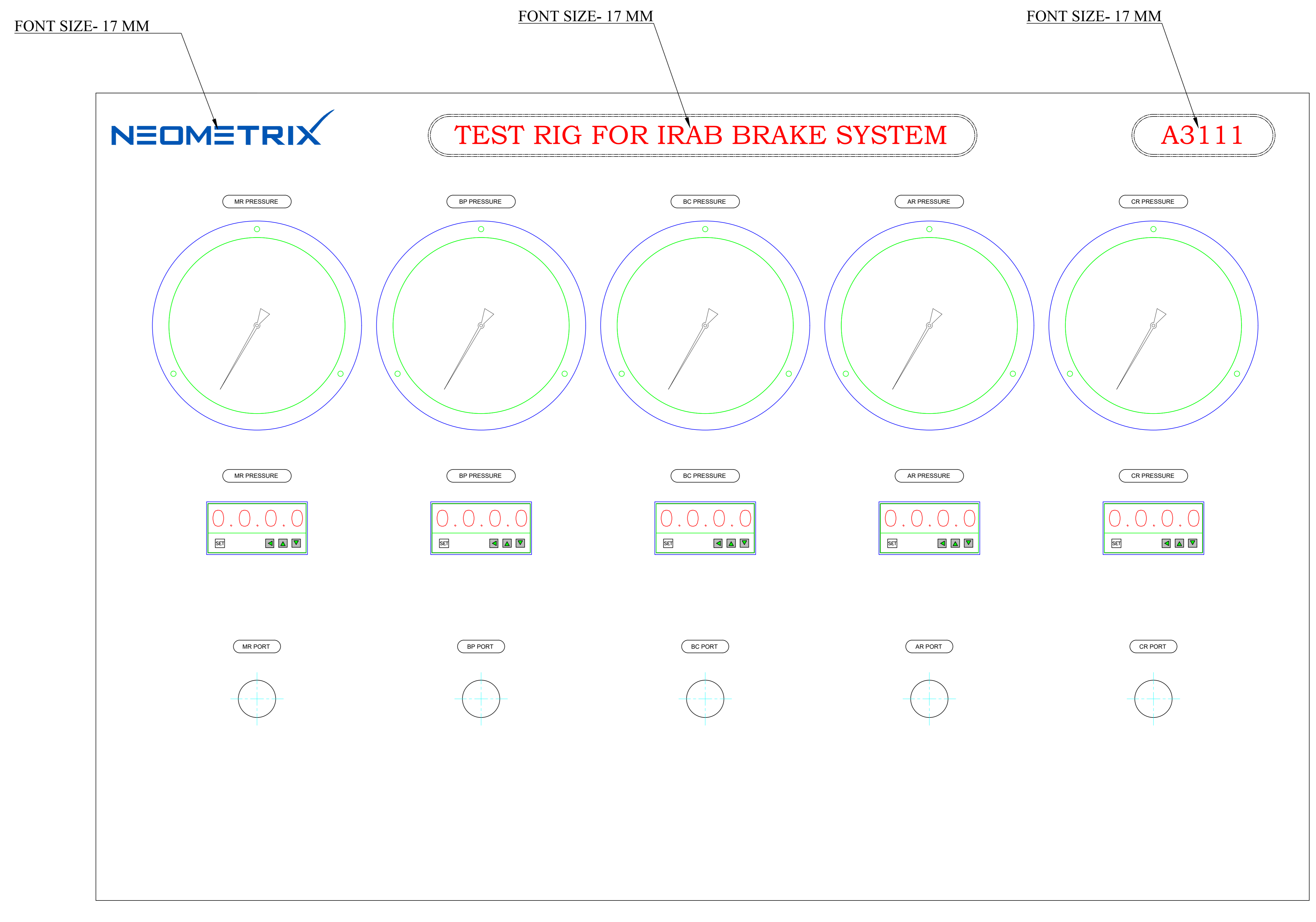
FRONT PANEL-1
