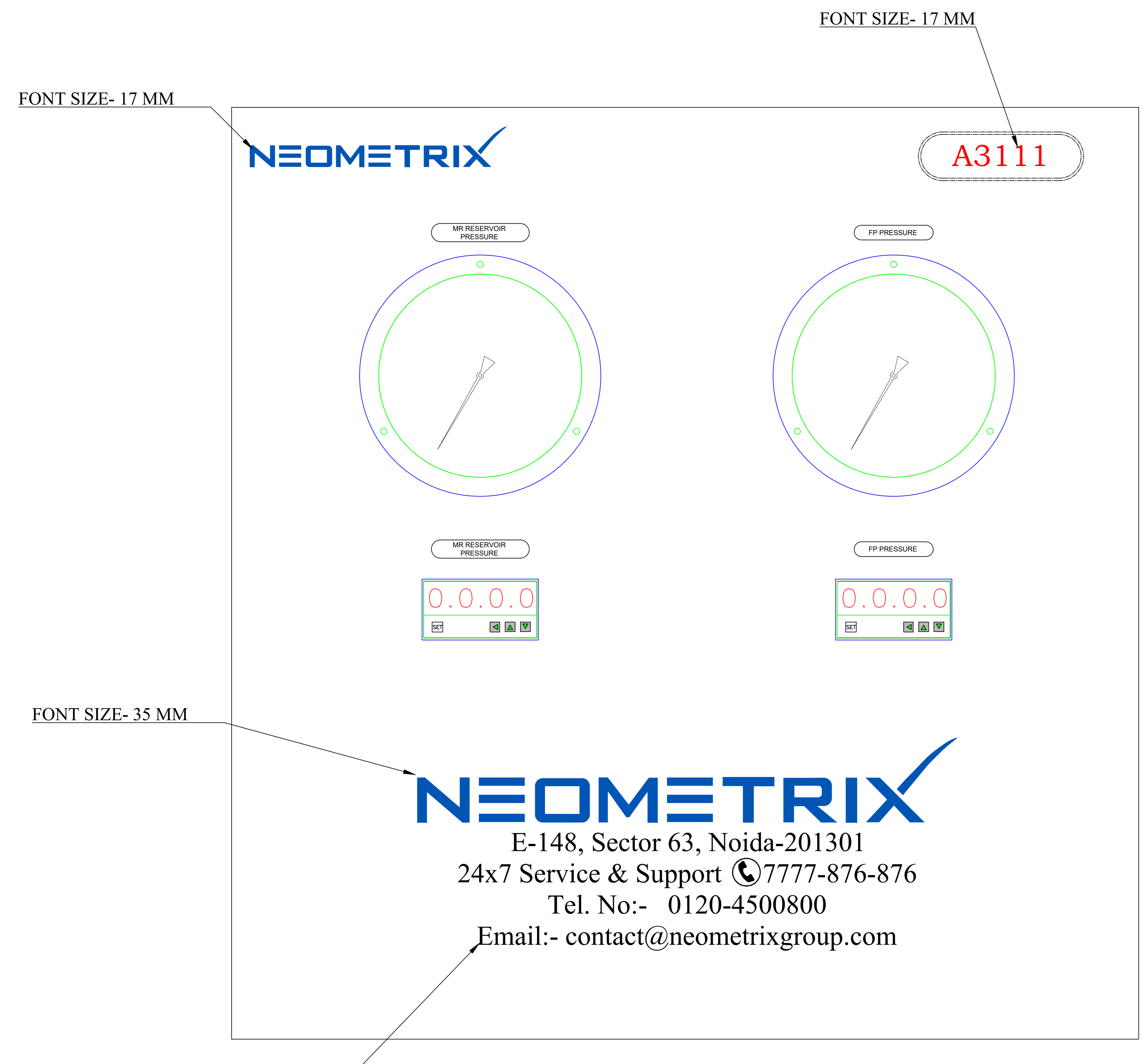
FRONT PANEL-2
