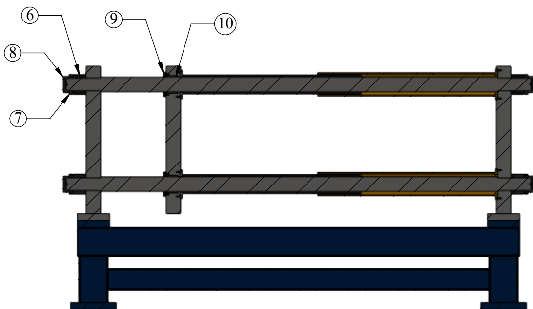
SECTION B-B
