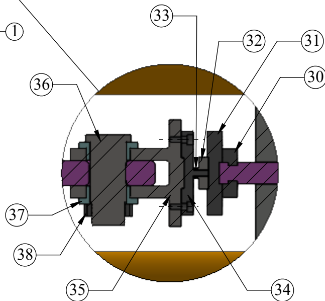
DETAIL E
