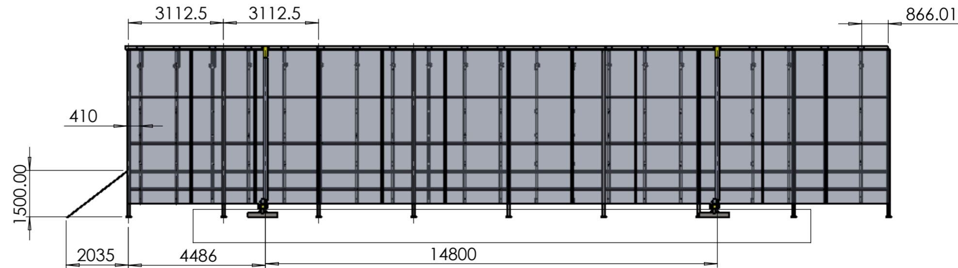
SIDE VIEW
